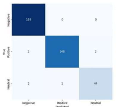
Figure 2. Confusion Matrix of the MARBERT Sentiment Model
