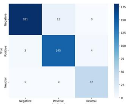
Figure 3. Confusion Matrix of the AraBERT Sentiment Model
